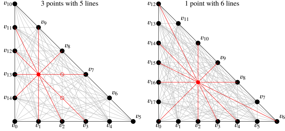
Fig. 3: The Wang-Shi split of degree 5, 6 with highlighted the intersection points with maximum degrees and the lines through one of them.
