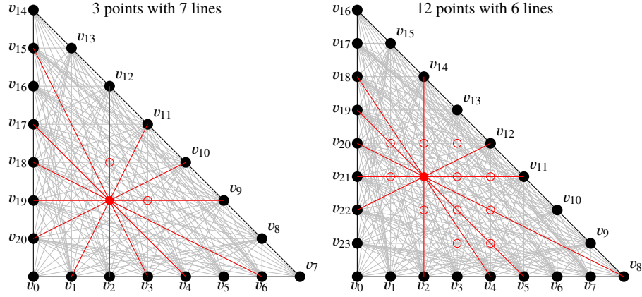
Fig. 4: The Wang-Shi split of degree 7, 8 with highlighted the intersection points with maximum degrees and the lines through one of them.
