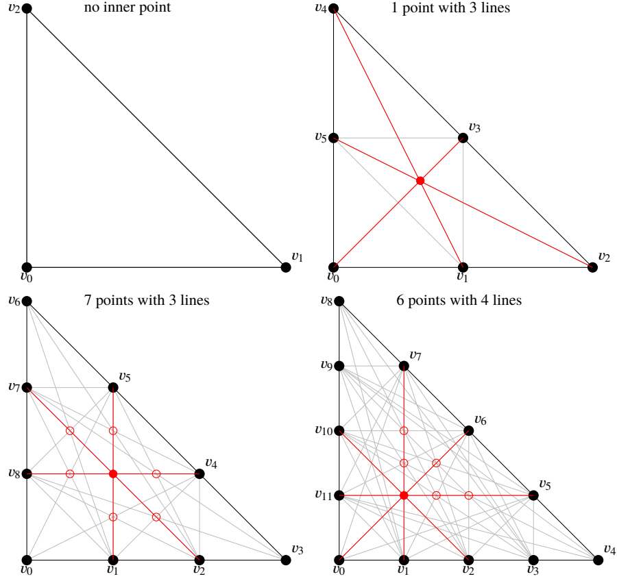
Fig. 2: The Wang-Shi split of degree 1–4 with highlighted the intersection points with maximum degrees and the lines through one of them.
