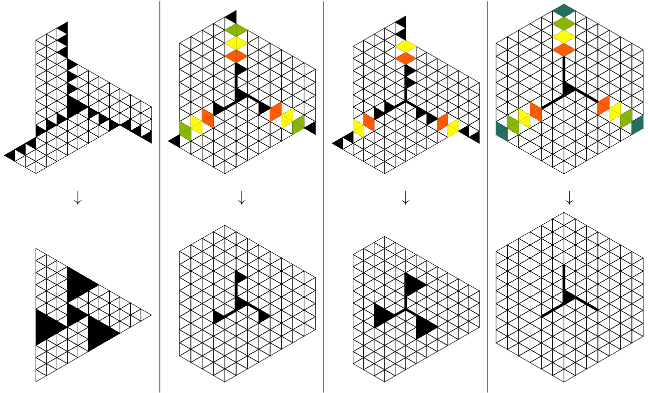
Figure 5: Selected examples of the region related to the determinant E_{s,t}^\mu(n) . From left to right (s, t, n, \mu) : (3, 0, 3, 4), (2, 1, 4, 3), (3, 1, 4, 2), (2, 2, 4, 3) . All regions are hexagonal after the forced tiling removal, except for the left-most one, which becomes triangular. The regions will typically have four triangular holes after the forced tiling removal. Exceptions are the right-most case, which has no mandatory points, and the one to its left, where the central hole has size 0.
