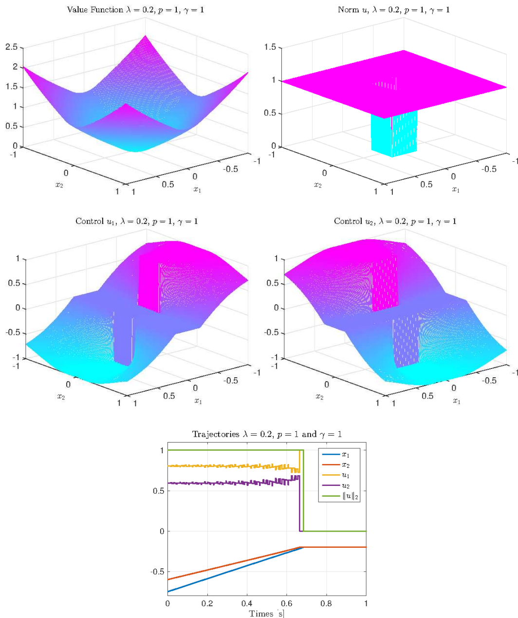
FIGURE 3. Infinite horizon control of the Eikonal dynamics with p = 1 . Row 1 and 2: value function V(x_1, x_2) , \|u\|_2 -norm of the optimal control, optimal controls u_1(x_1, x_2) and u_2(x_1, x_2) , over the state space \Omega = [-1, 1]^2 . Row 3: trajectories for the initial condition (x_1(0), x_2(0)) = (-0.75, -0.6) .
