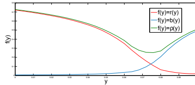
FIG. 5. Example II: Red and blue particle density as well as their sum \rho at time T = 100 in case of non-equal initial mass.
