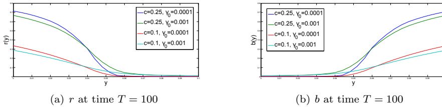
FIG. 4. Example II: Red and blue particle density in y -direction at time T = 100 .
