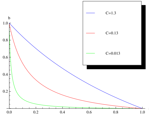
FIG. 1. Stationary solution curves for \gamma_1 = 0.5 , \gamma_2 = 0.4 and \gamma_0 = 0.001
