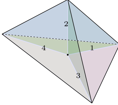
FIGURE 5. Clough–Tocher split.
