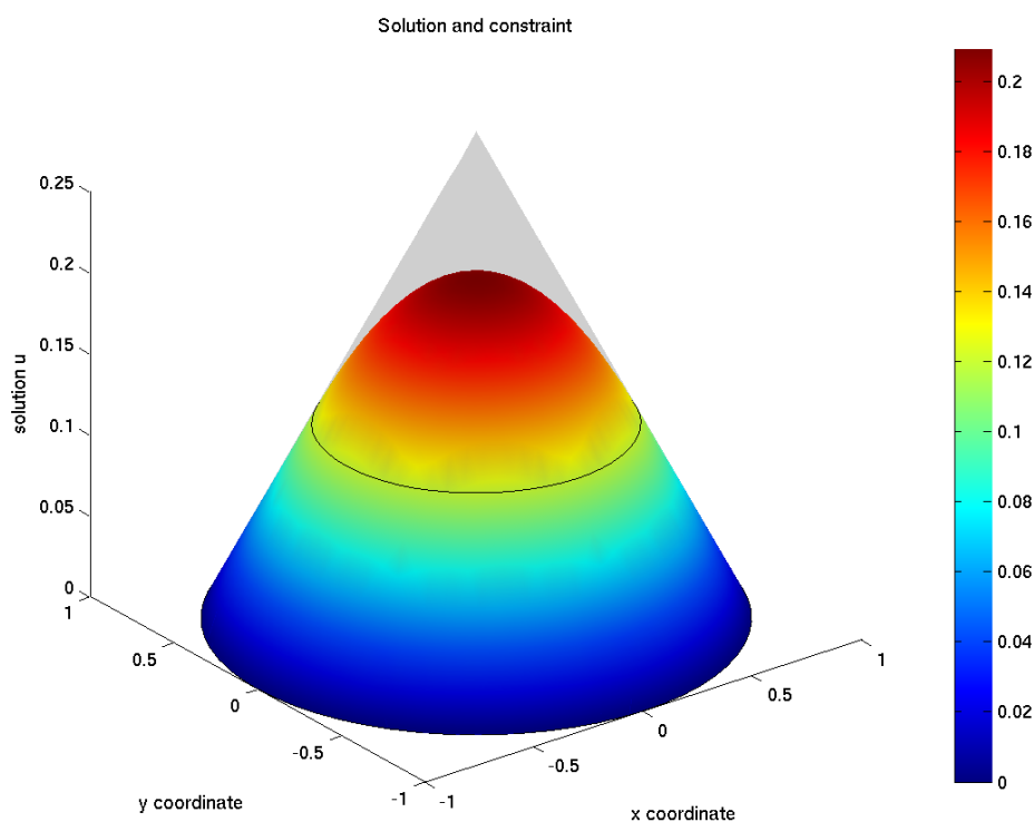
FIGURE 4.3. The figure shows the final iterate u_\gamma for Example 4.3. The constraint cone is superimposed on the solution. The contour line marks the boundary of the active set.
