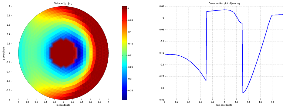
FIGURE 4.5. The figure shows the value of |\nabla u_\gamma| - g for the final iterate of Example 4.4 on the domain (left), and its cross section along the first median for \gamma = 10^2 (right).
