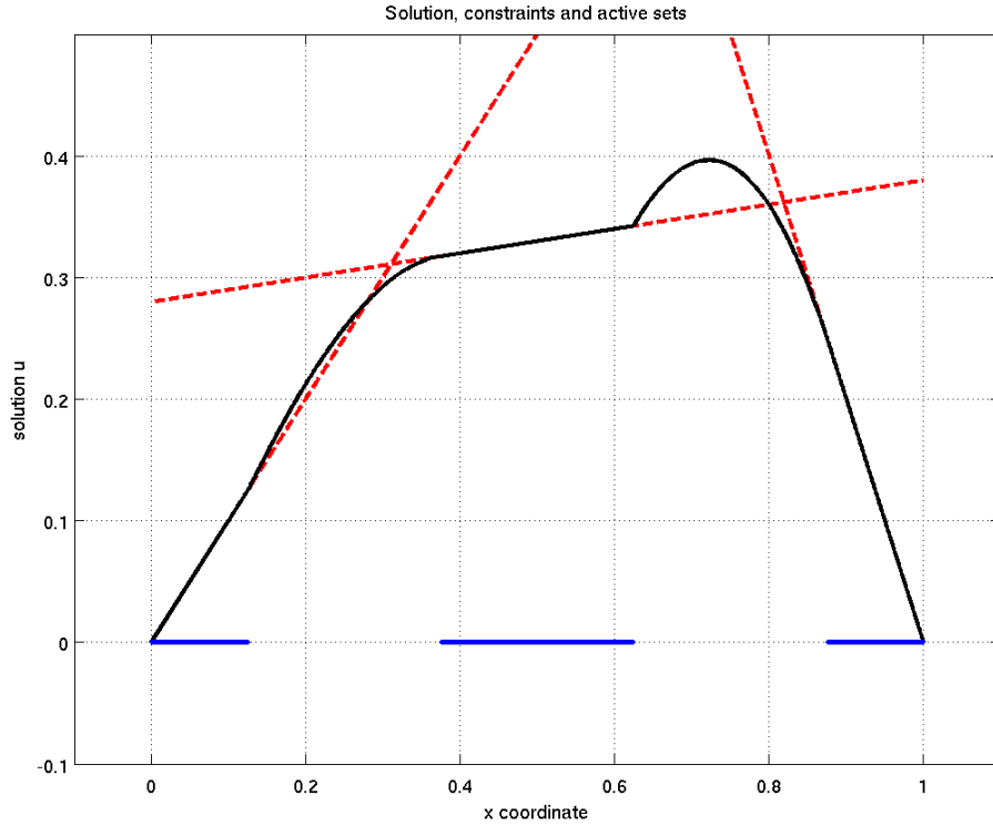
FIGURE 4.2. The figure shows the final iterate u_\gamma for Example 4.2. The active sets are again depicted in blue on the x -axis, and A^+ (left and middle) is disconnected. The dashed red lines represent the constraint envelope.
