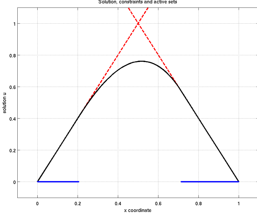
FIGURE 4.1. The figure shows the final iterate u_\gamma for Example 4.1. The active sets A^+ (left) and A^- (right) are depicted in blue on the x -axis. The dashed red lines represent the constraint envelope.
