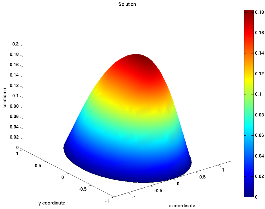
FIGURE 4.4. The figure shows the final iterate u_\gamma for Example 4.4.
