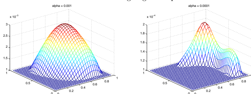
FIGURE 5.1. Lagrange multiplier
