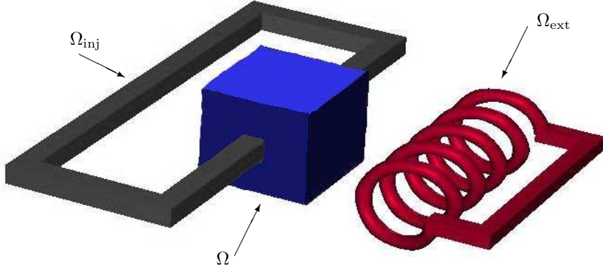
FIGURE 3.1. General Setup: Fluid region \Omega (cube), external conductor \Omega_{\text{inj}} attached to the fluid region, and external conductor \Omega_{\text{ext}} separate from the fluid region.
