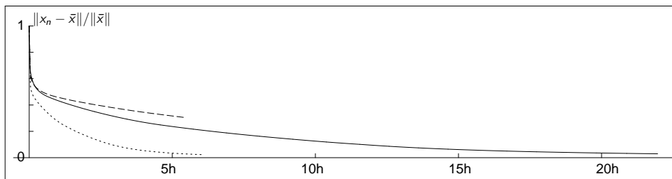
FIGURE 4 The different convergence rates of the thresholded Landweber algorithm (solid line), the projected Landweber algorithm (dashed line) and the projected steepest descent algorithm (dotted line), for the third example. The projected steepest descent algorithm converges about four times faster than the thresholded Landweber iteration. The projected Landweber iteration does better at first (not visible in this plot), but loses with respect to iterative thresholding afterwards. The horizontal axis has time (in hours), the vertical axis displays the relative error.
